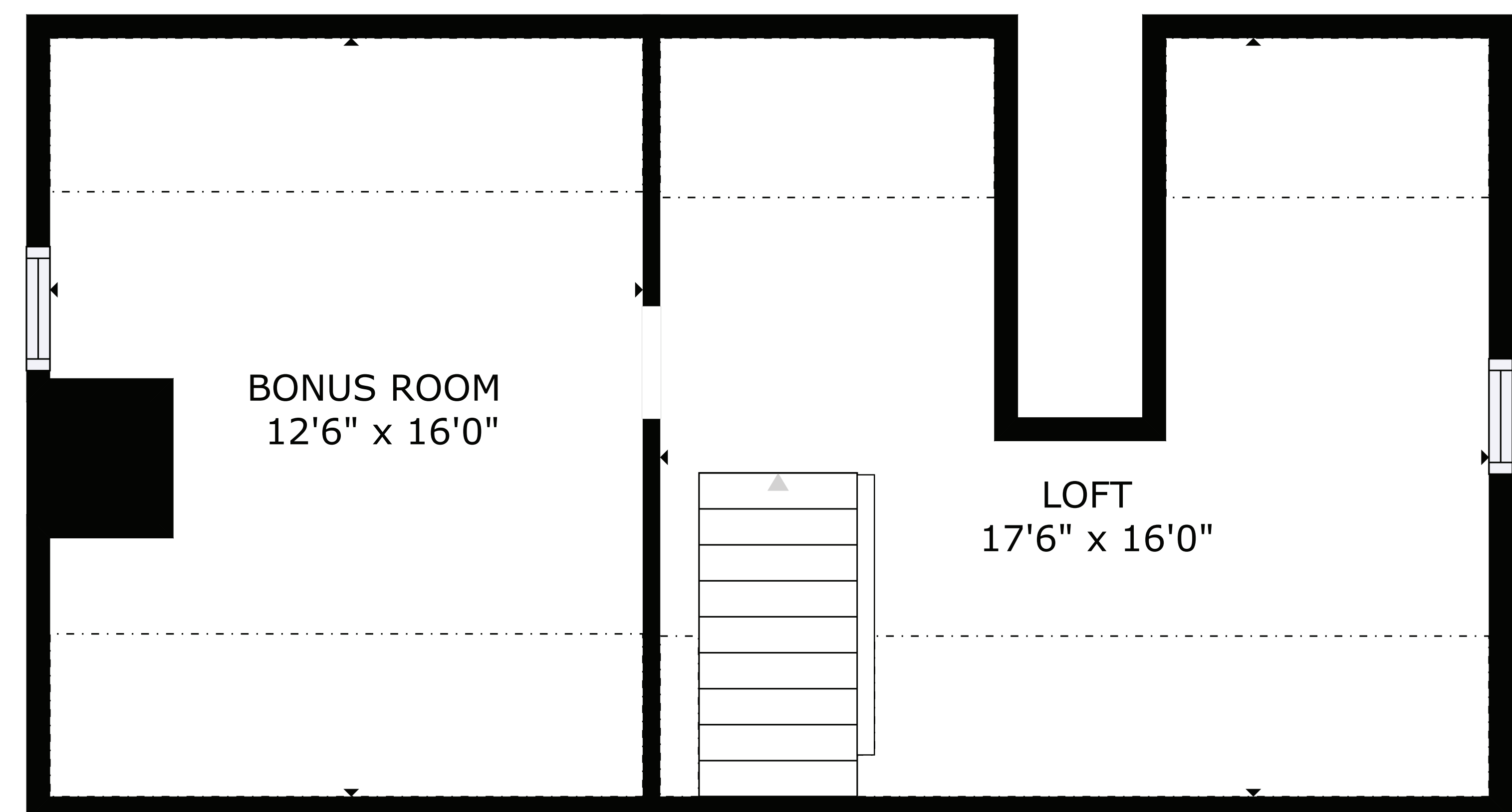
FLOOR 3
