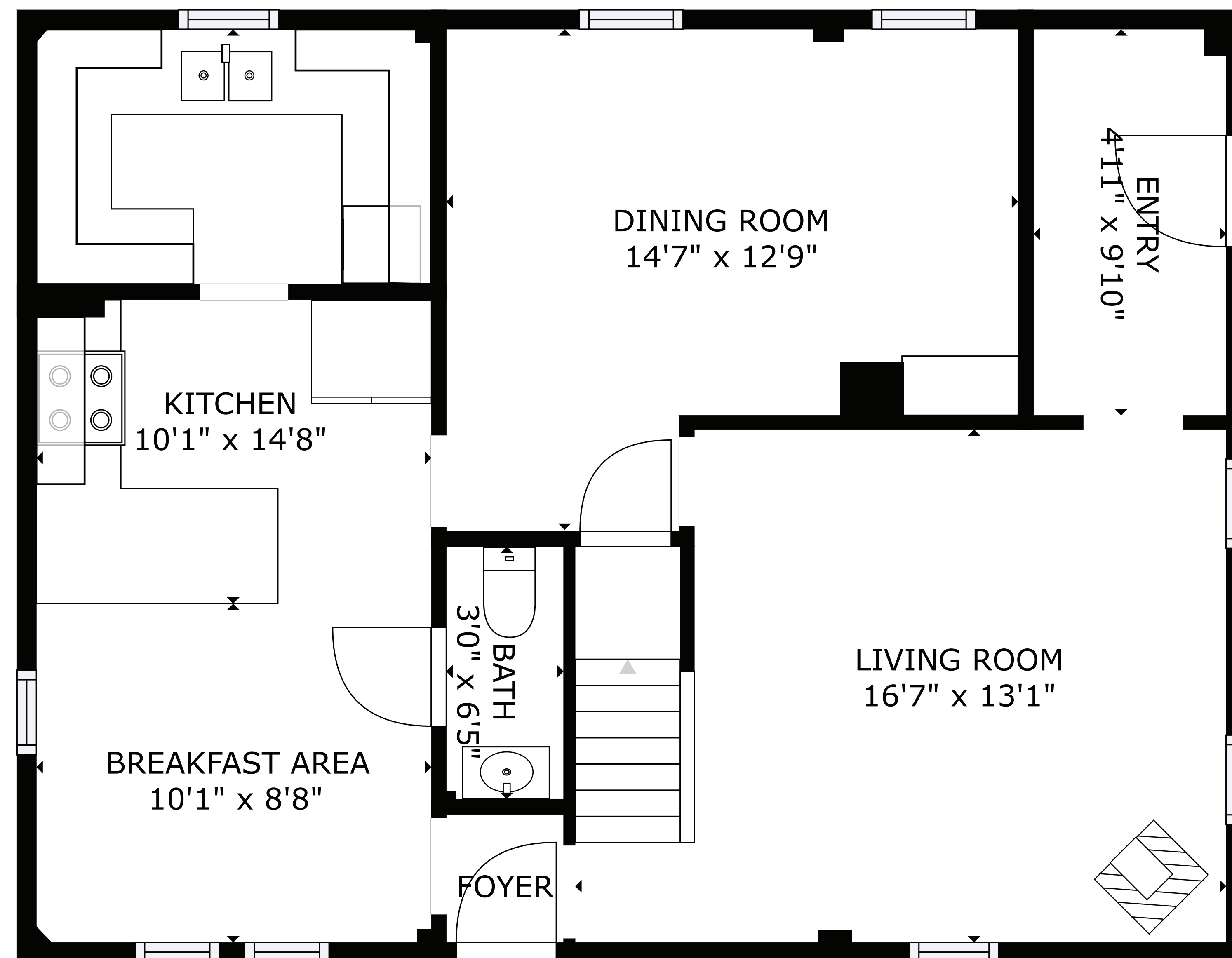
FLOOR 1
