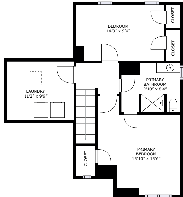
LOWER LEVEL
