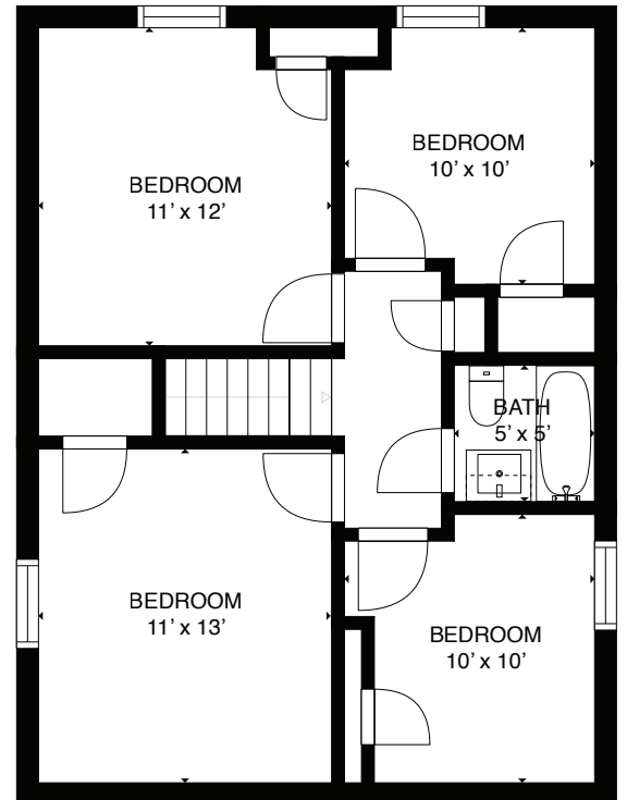
Second Level
