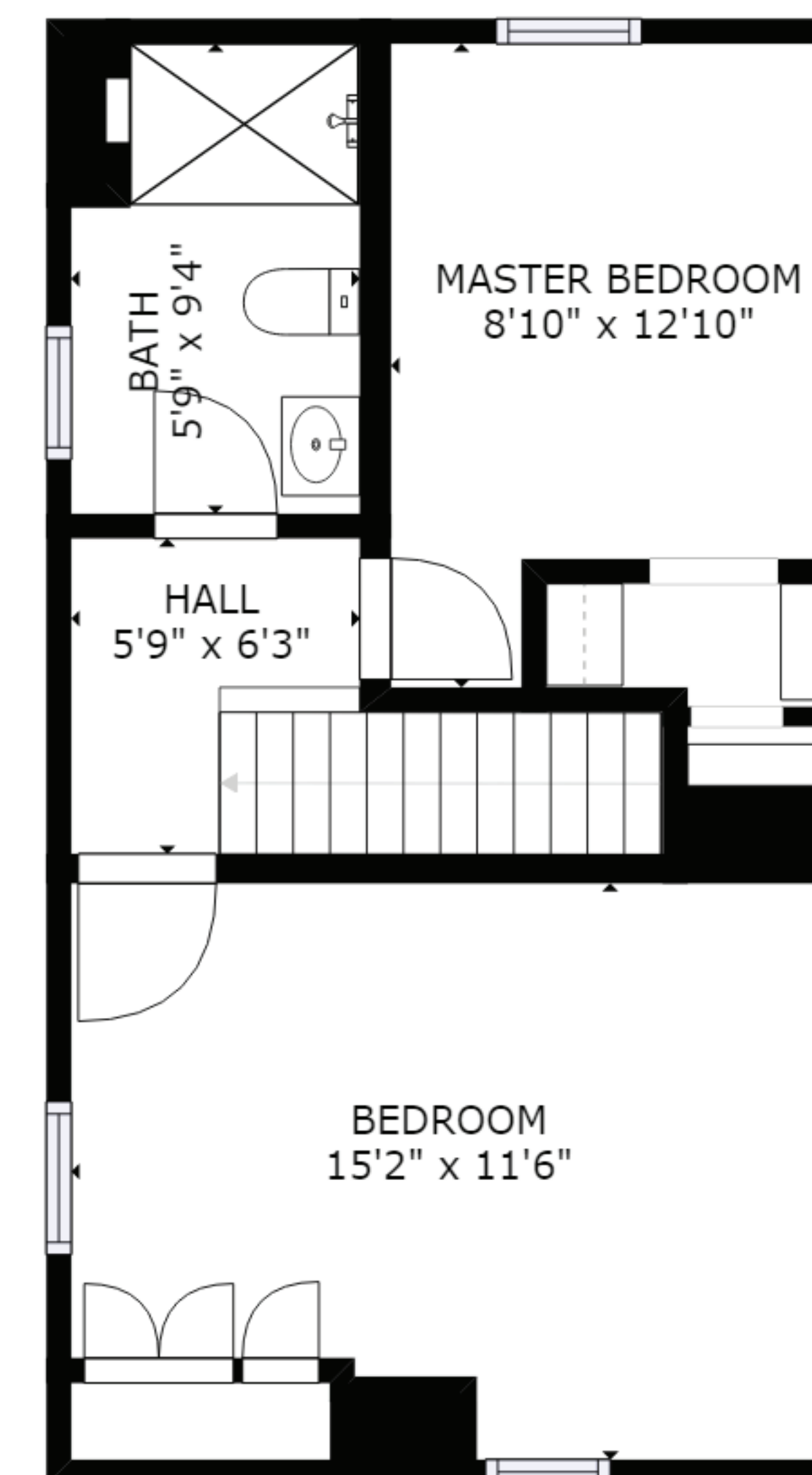
FLOOR 3
