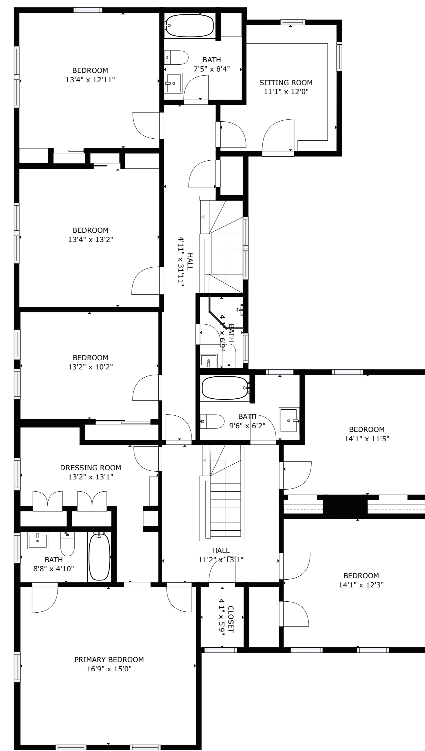
FLOOR 3
