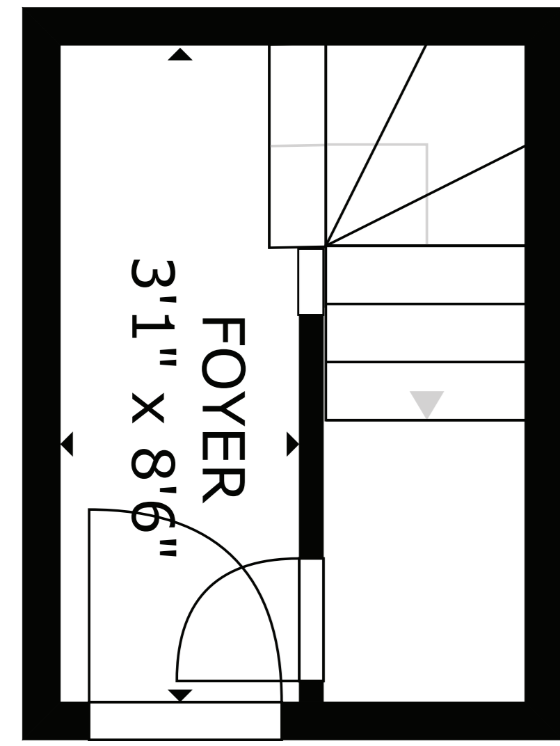
FLOOR 1
