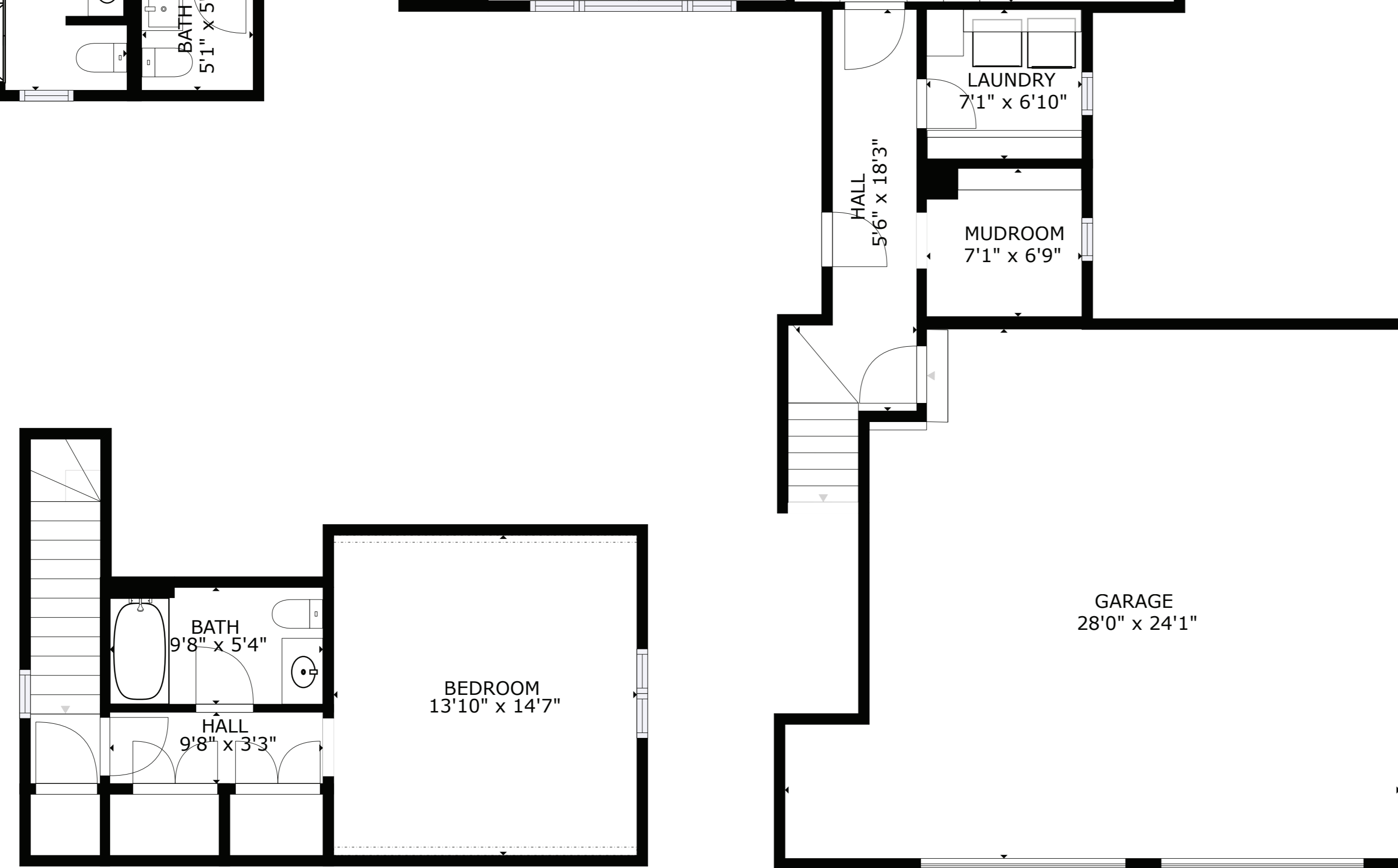
FLOOR 2
