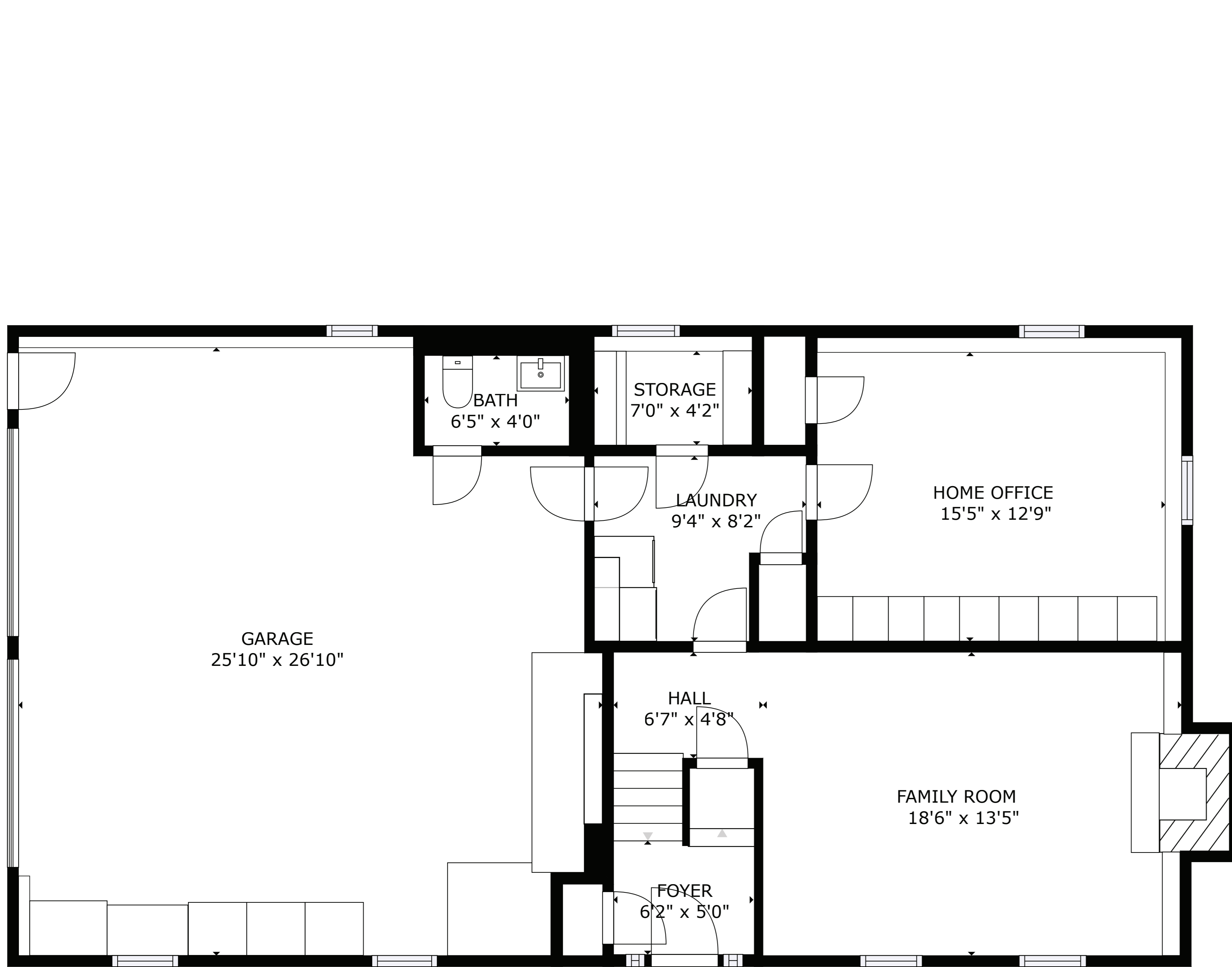
FLOOR 1
