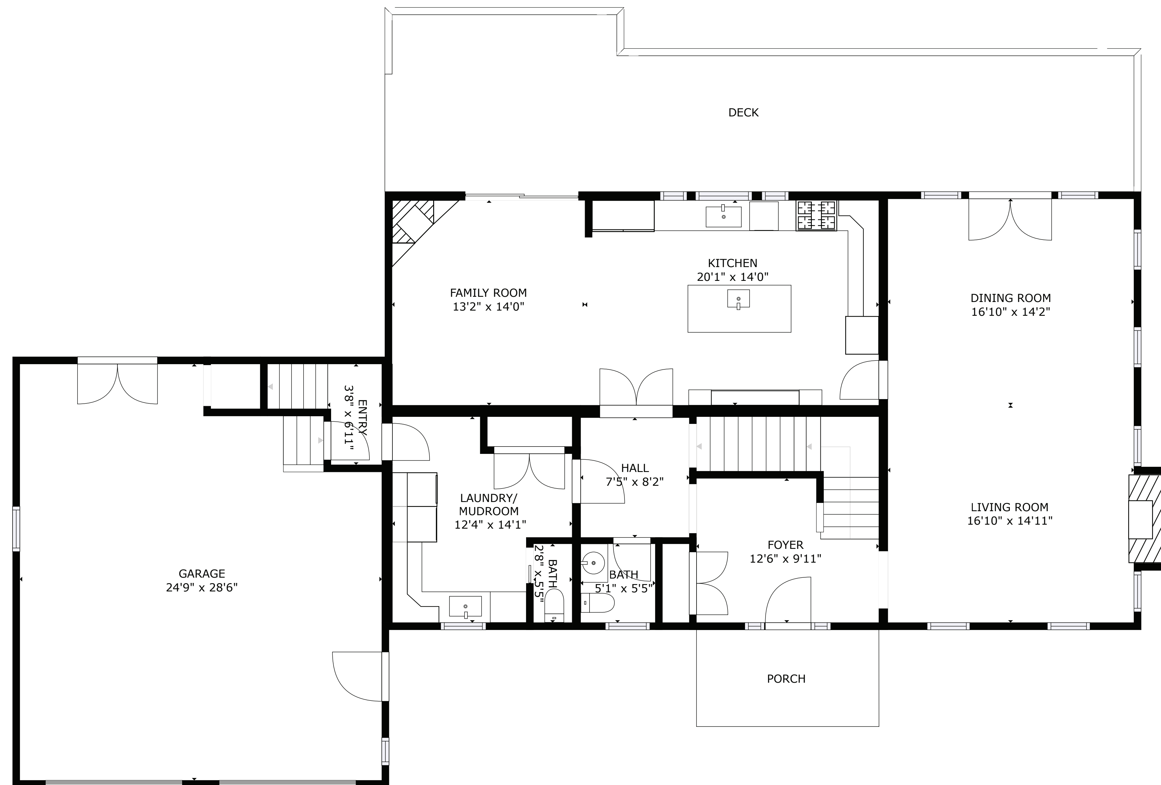
FLOOR 2
