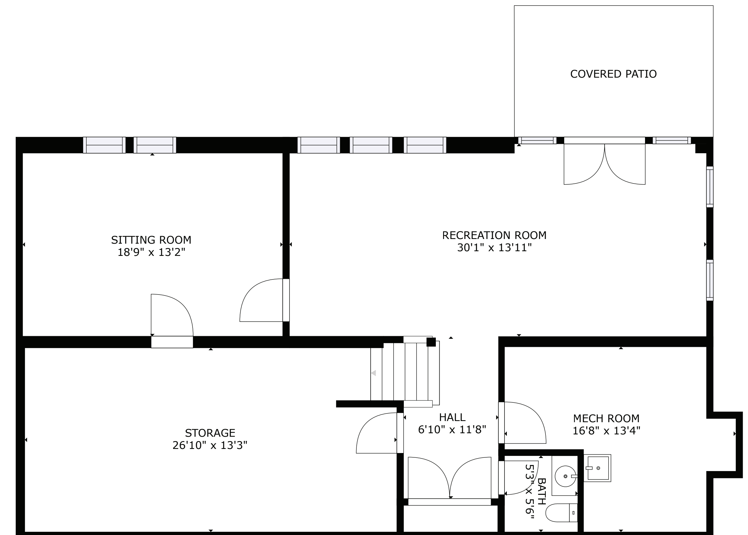
FLOOR 1
