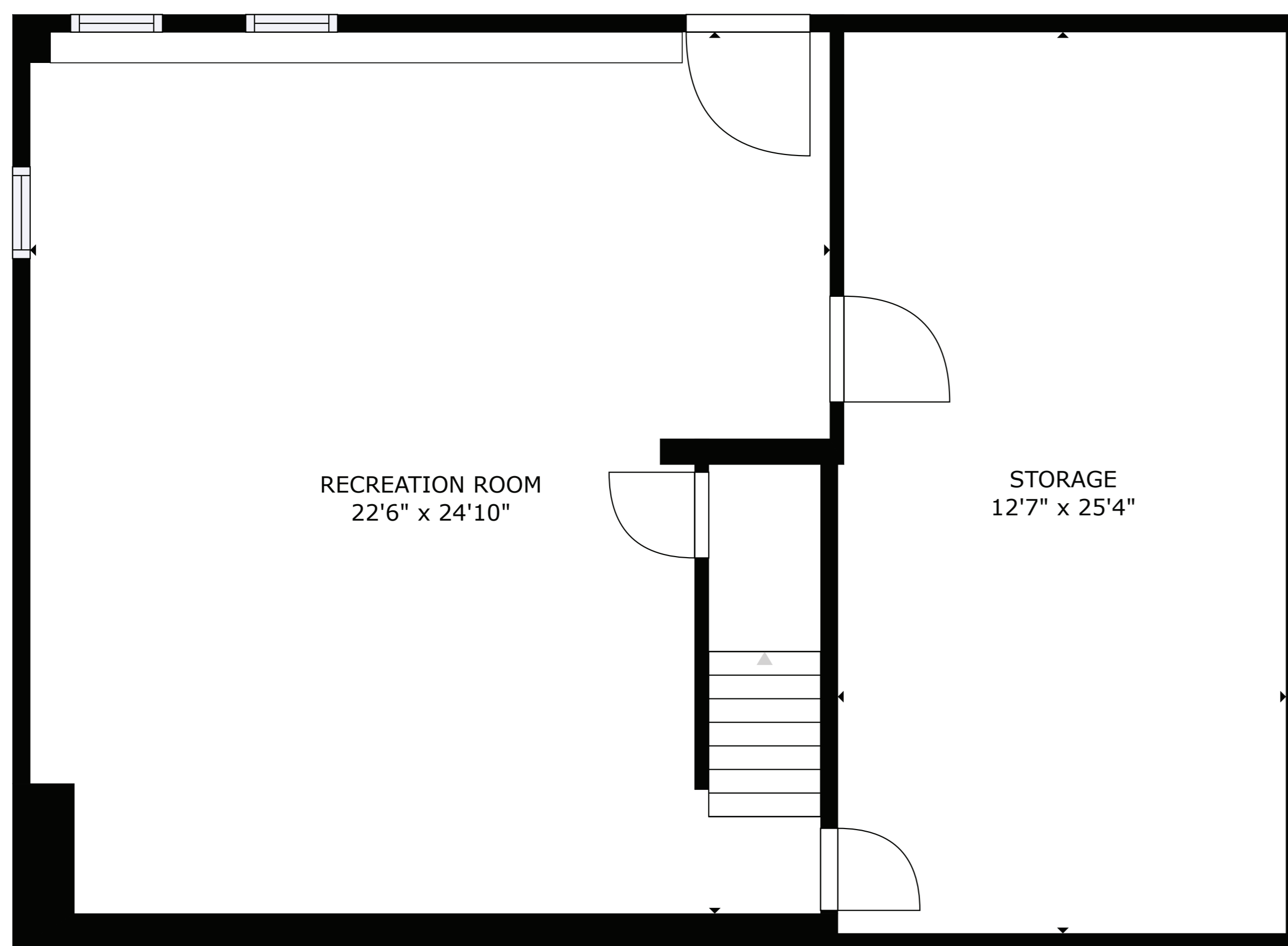
FLOOR 1
