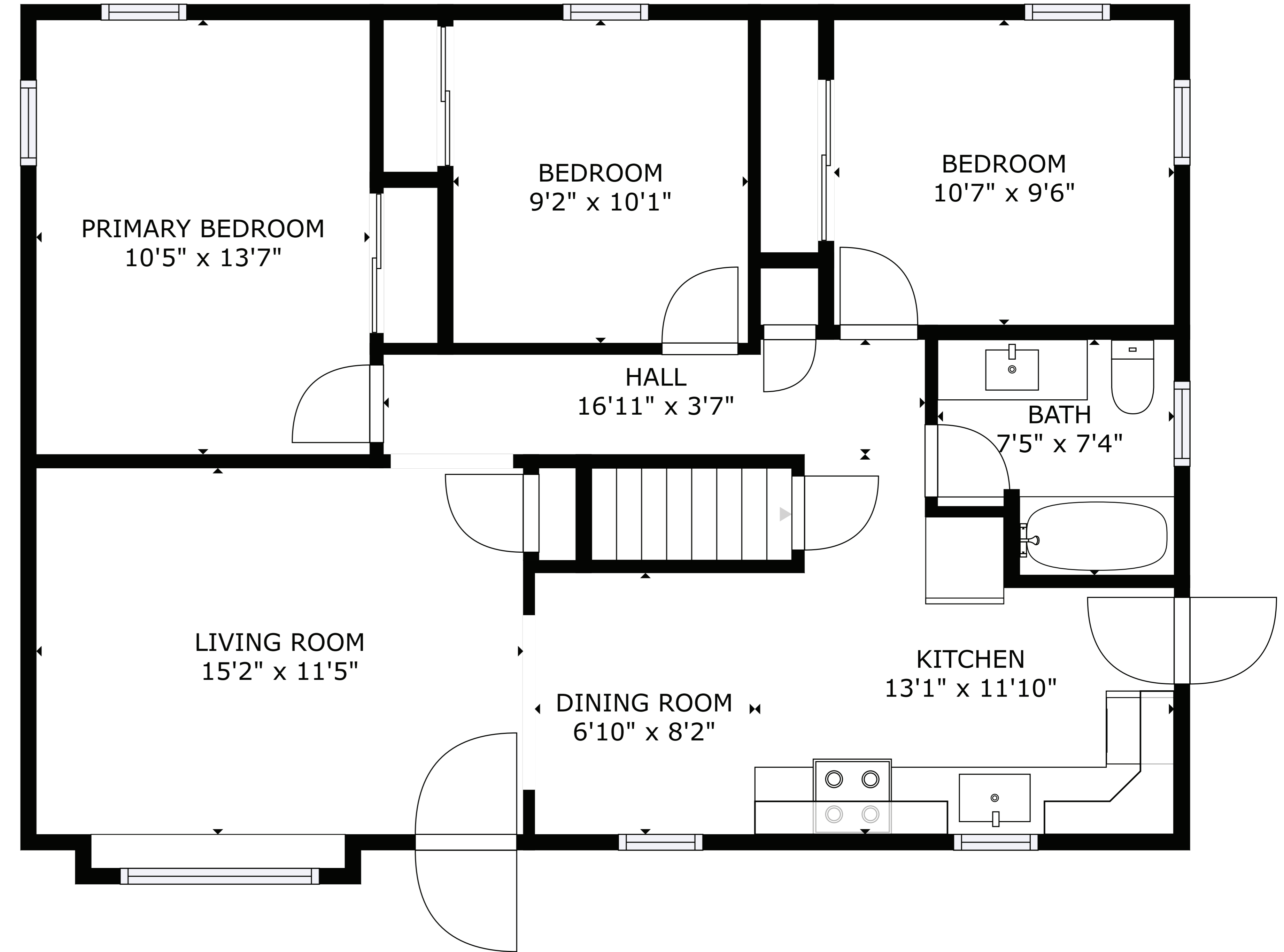
FLOOR 2
