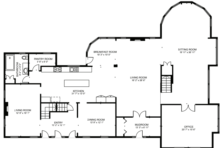
FLOOR 2
