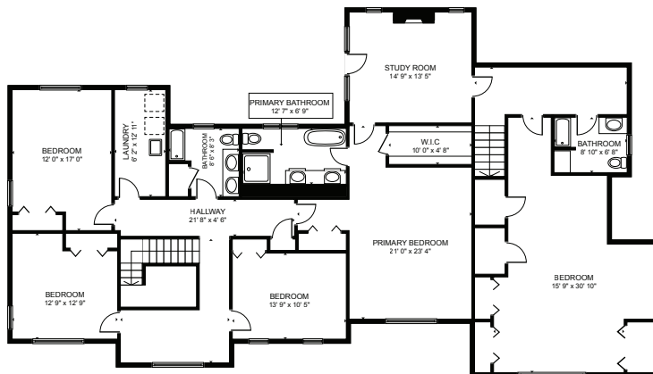
FLOOR 3
