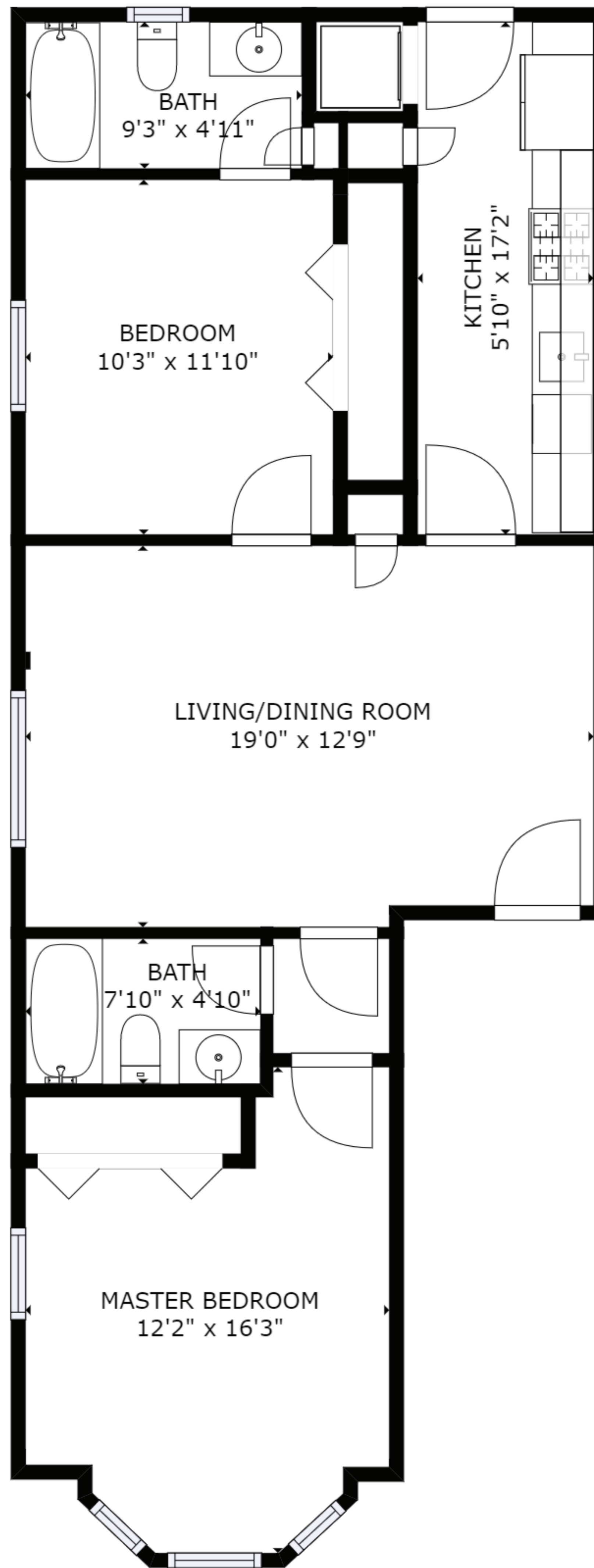
FLOOR 1
