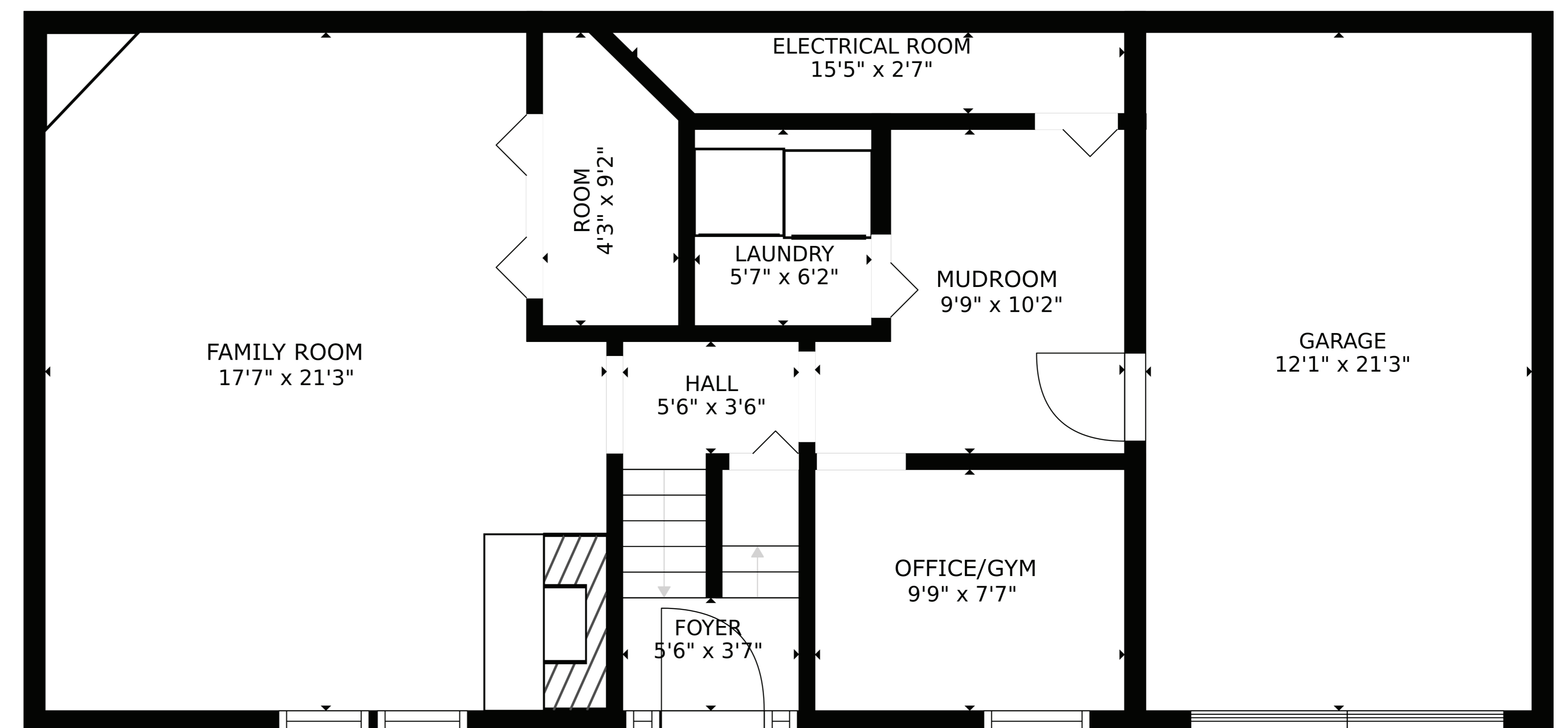
FLOOR 1
