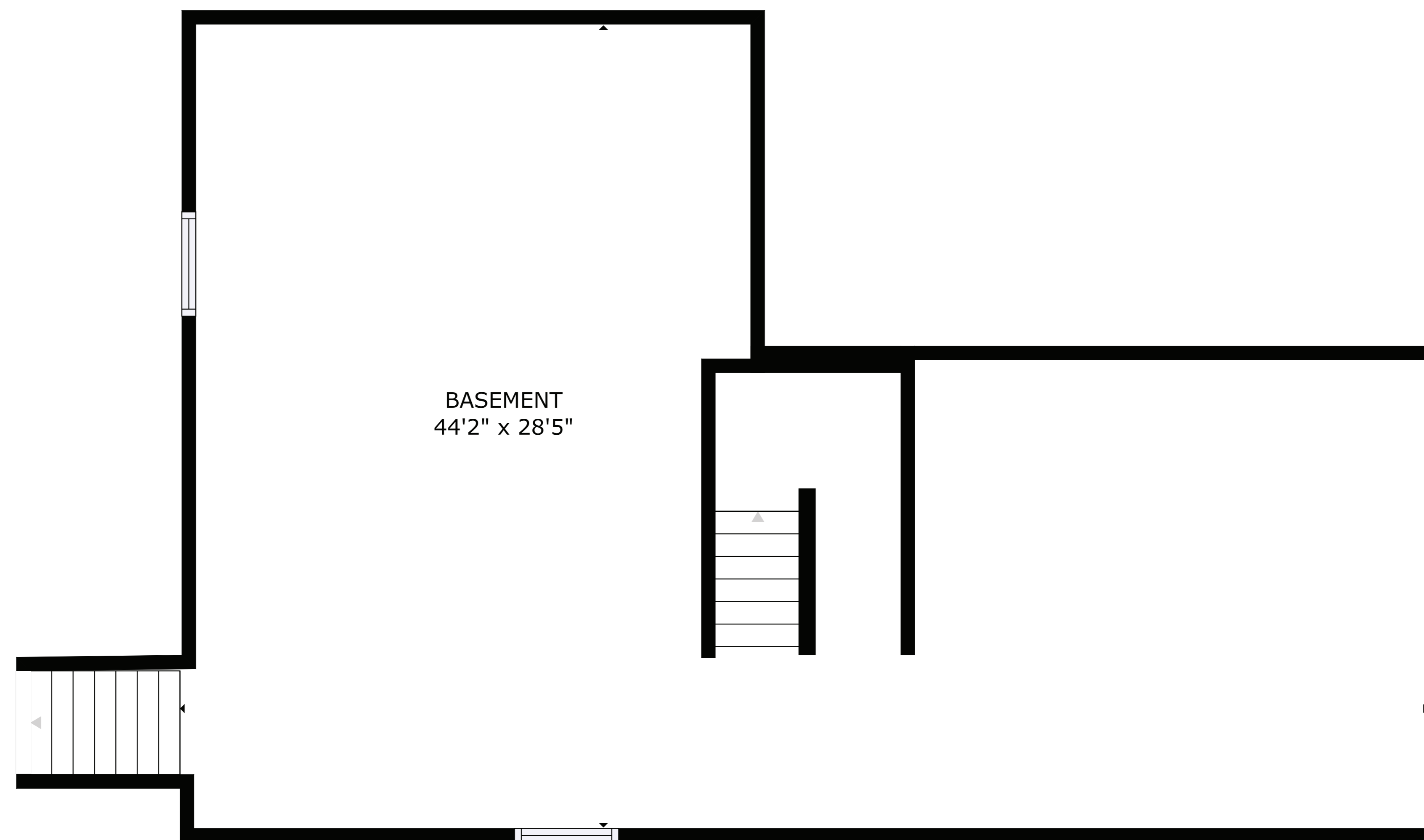
FLOOR 1
