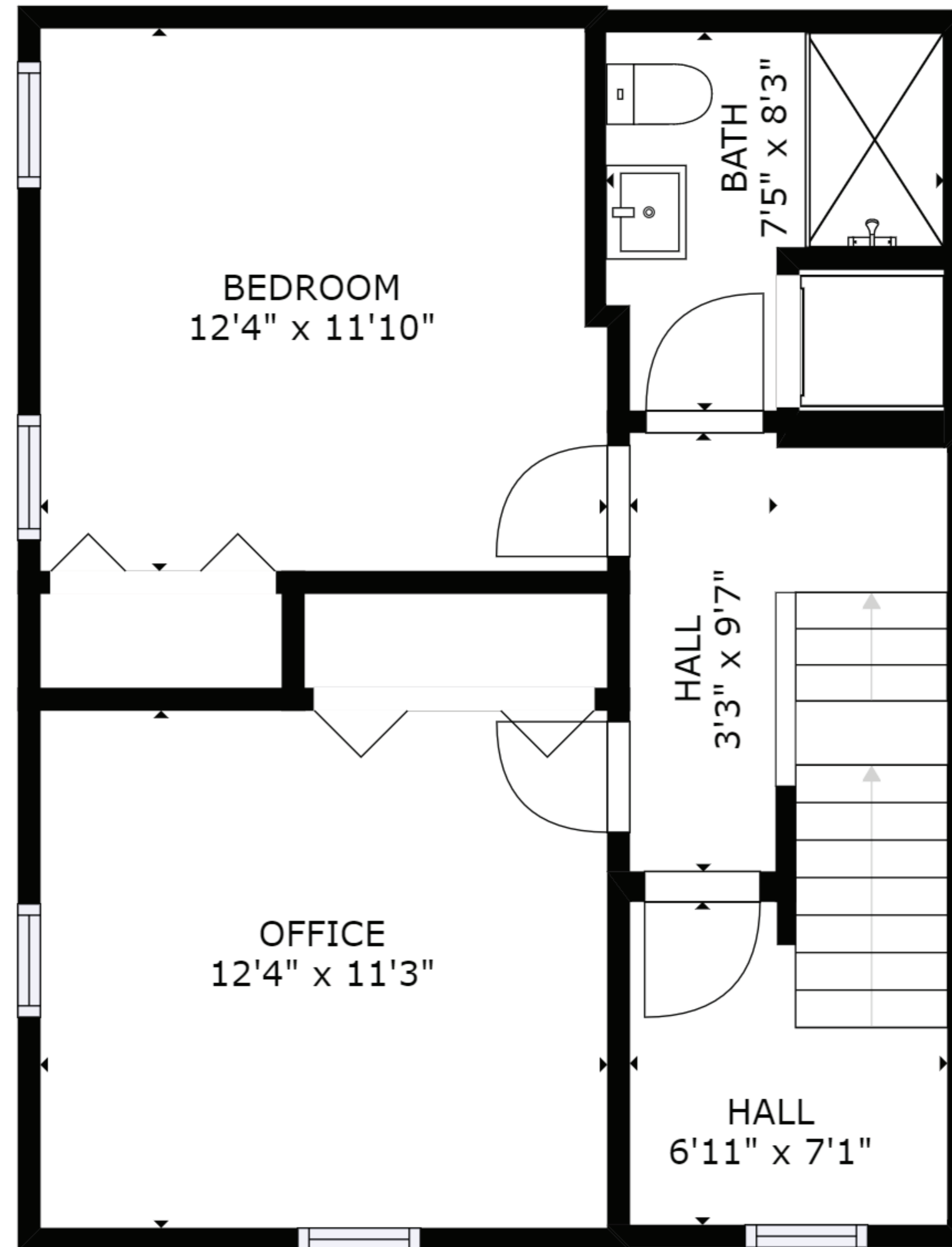
FLOOR 2
