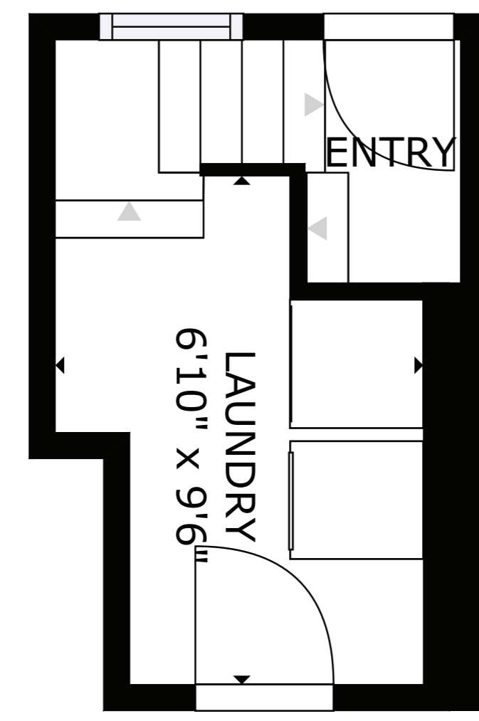
FLOOR 1
