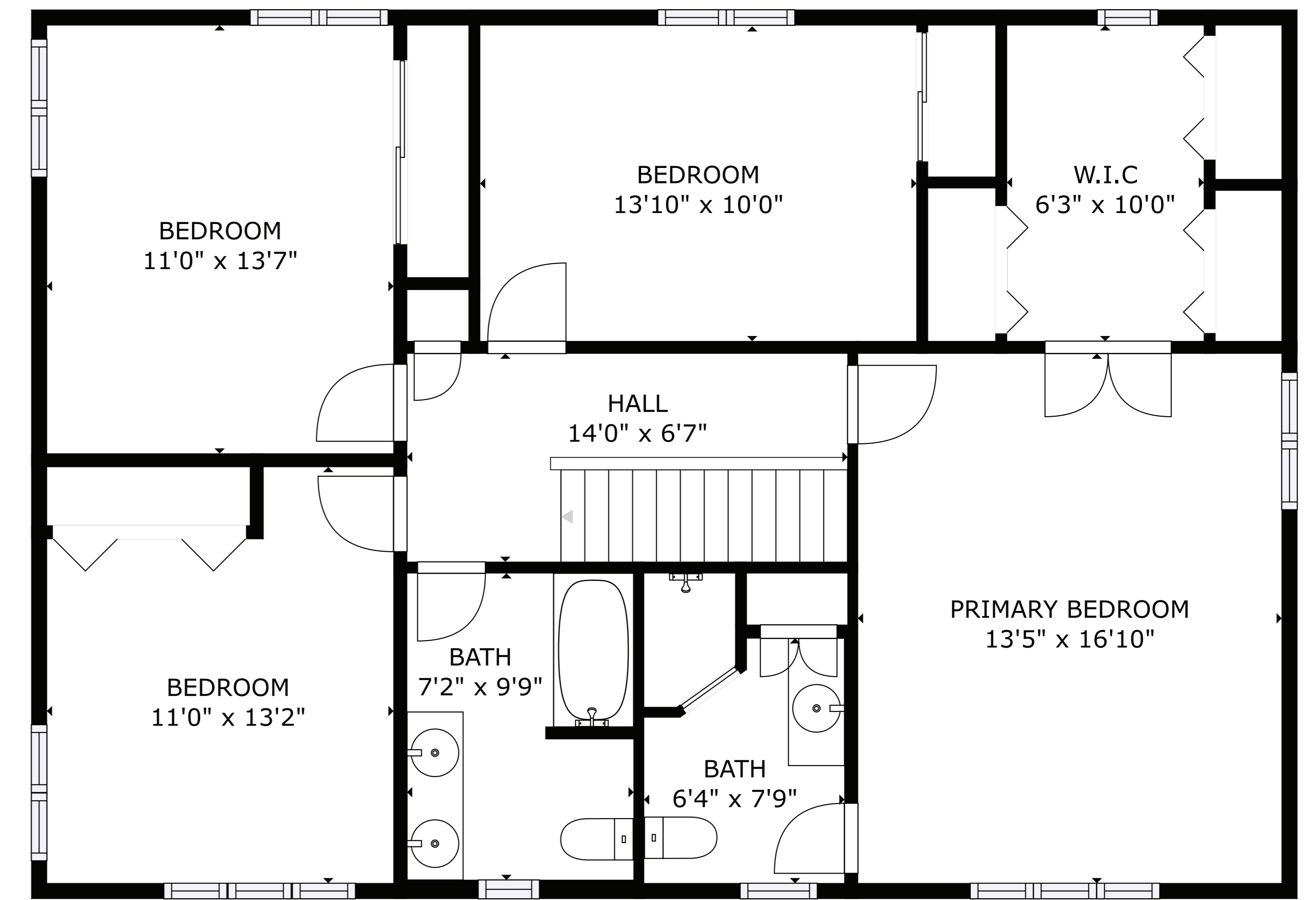
FLOOR 3
