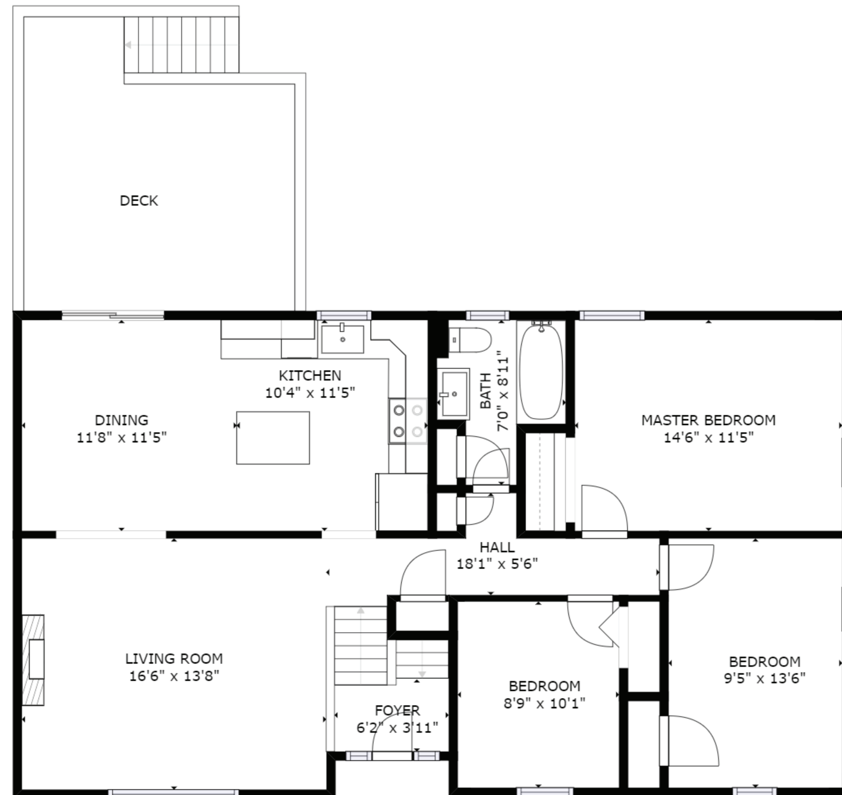
FLOOR 2
