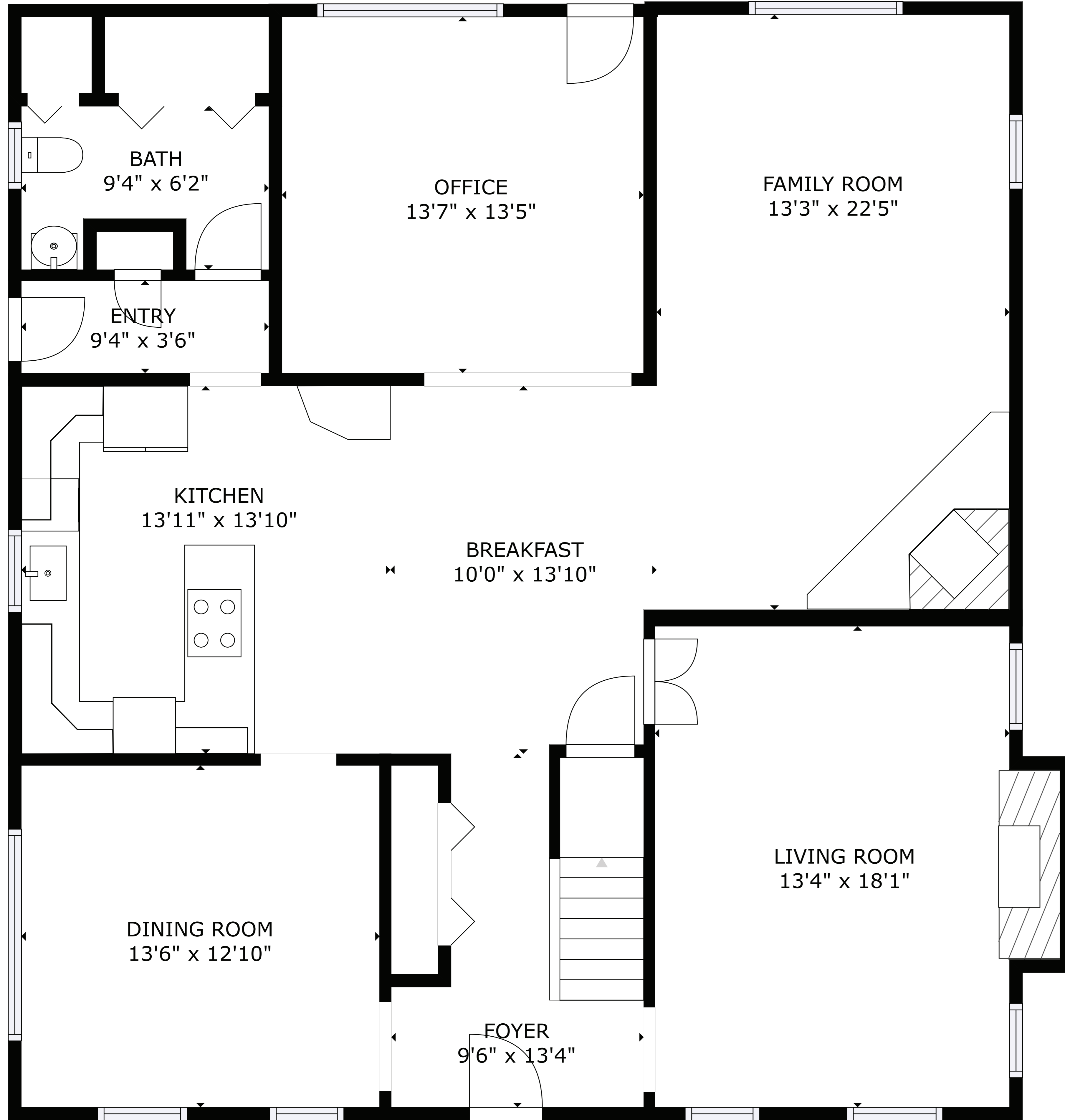
FLOOR 1
