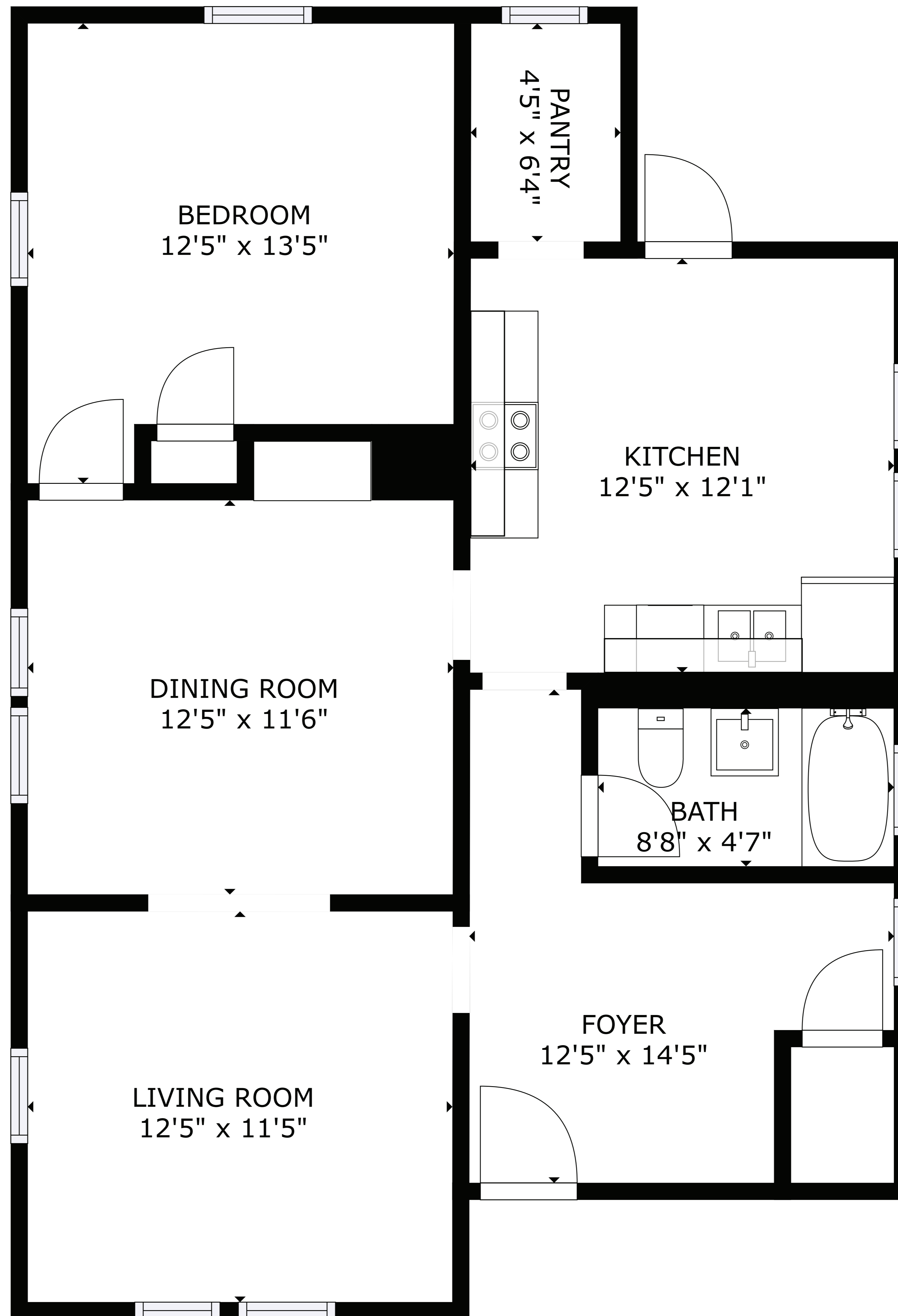
FLOOR 1
