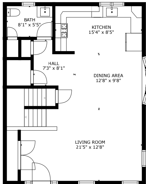
Main Level
