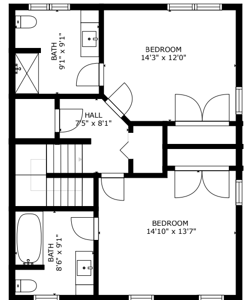
Second Level
