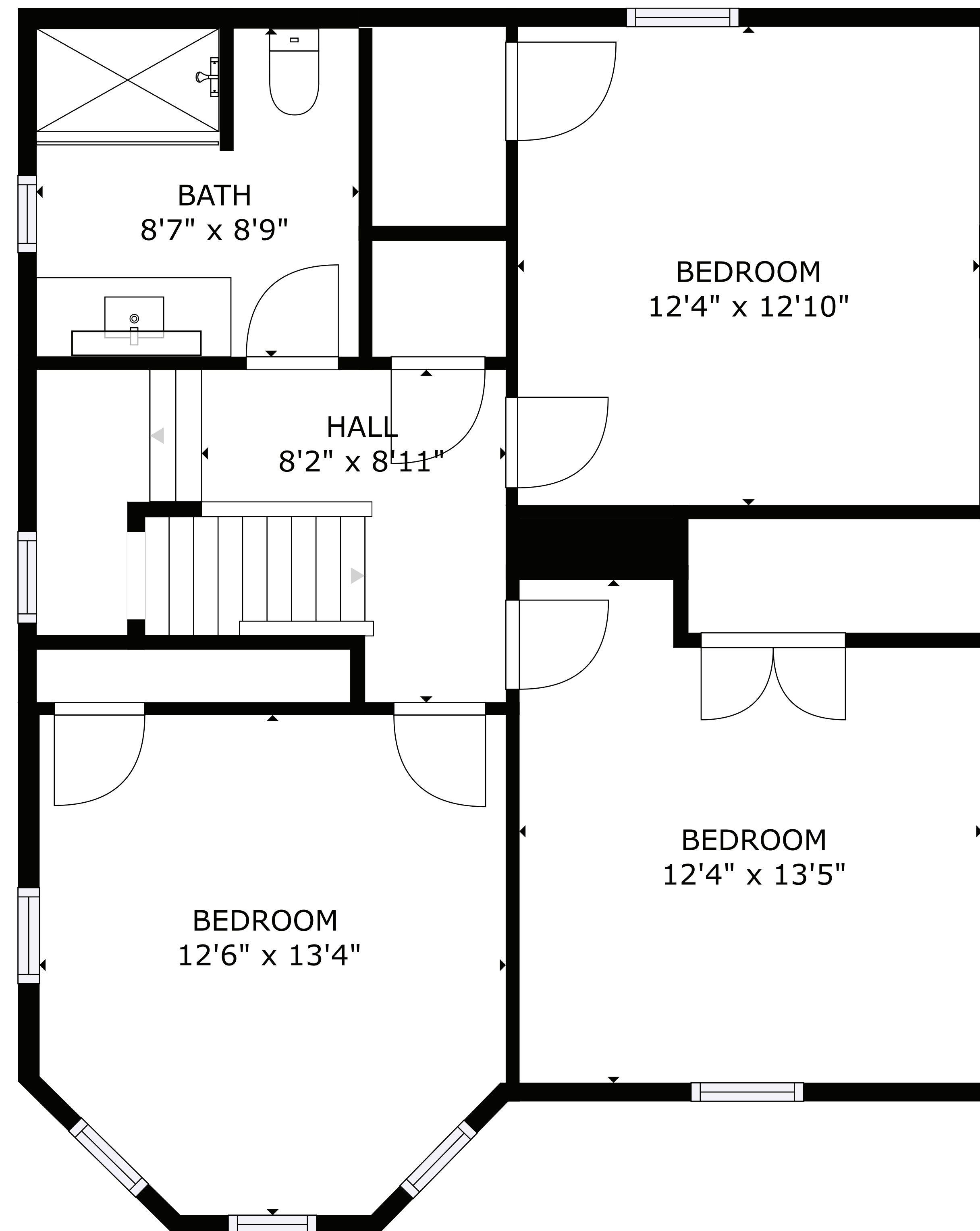
FLOOR 2
