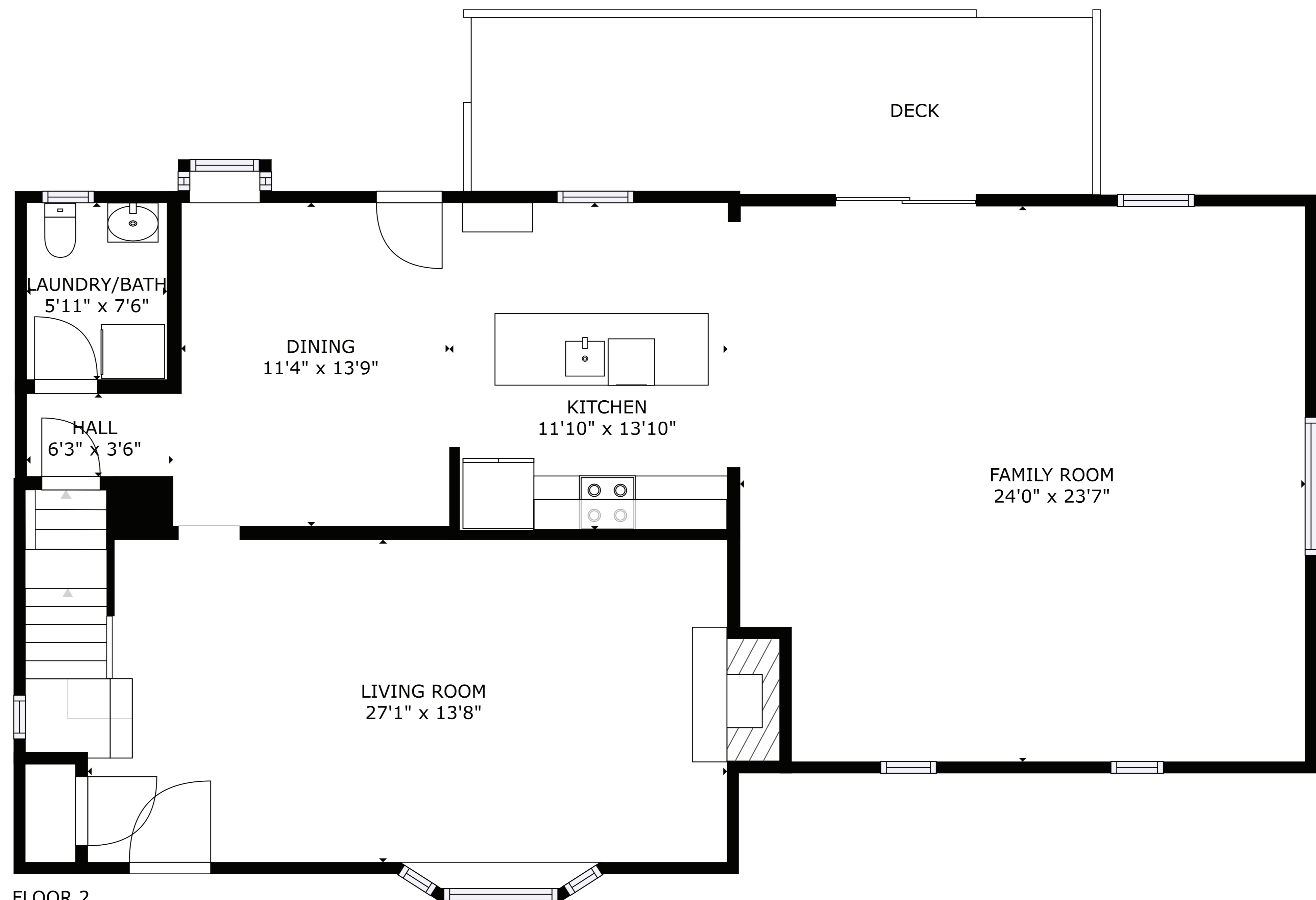
FLOOR 2
