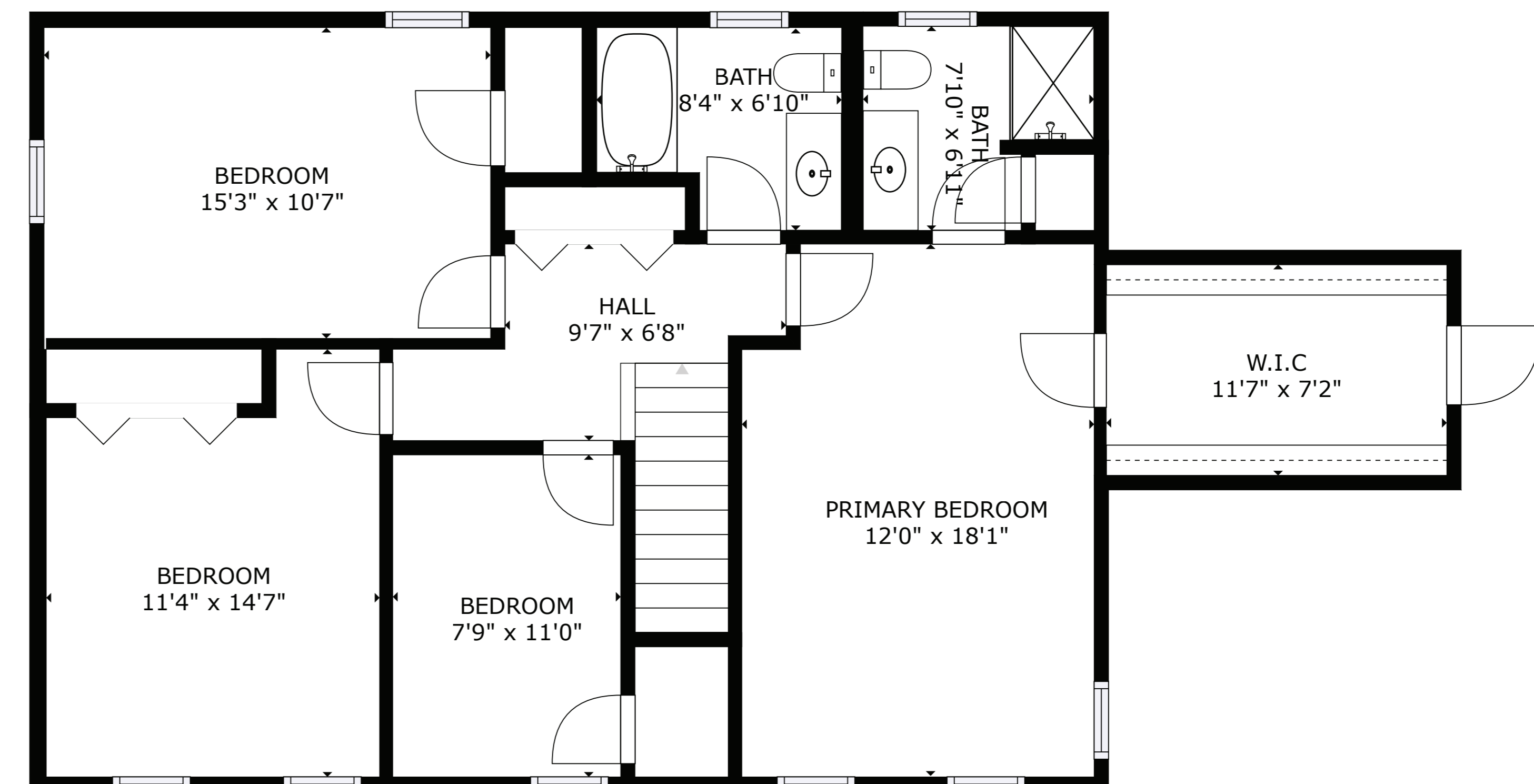
FLOOR 3
