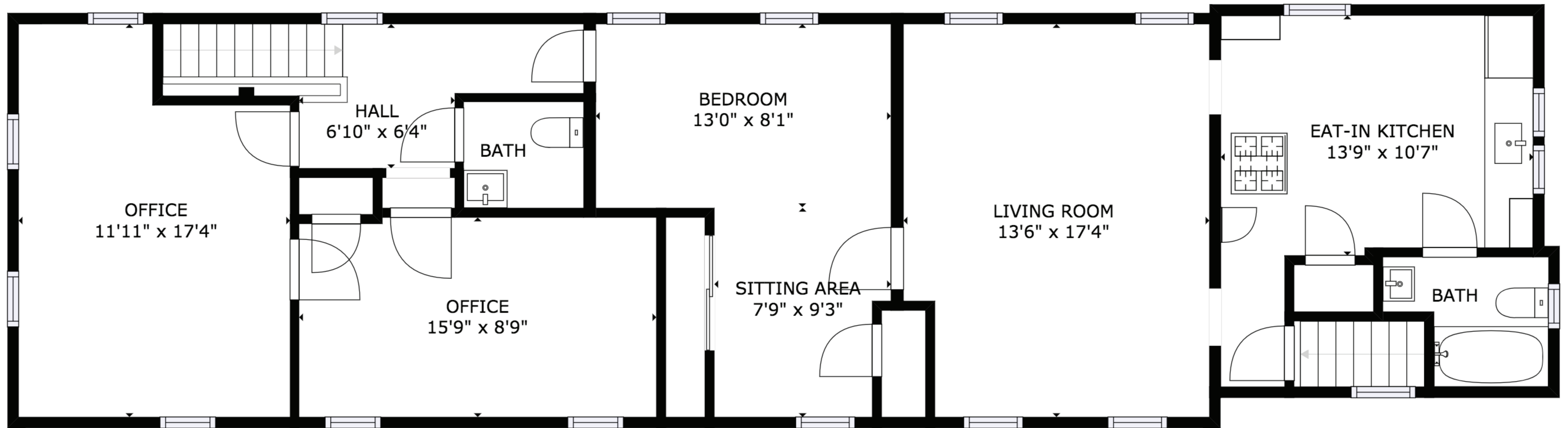
FLOOR 2
